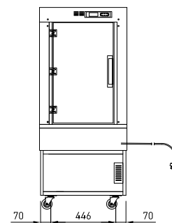
REAR VIEW
